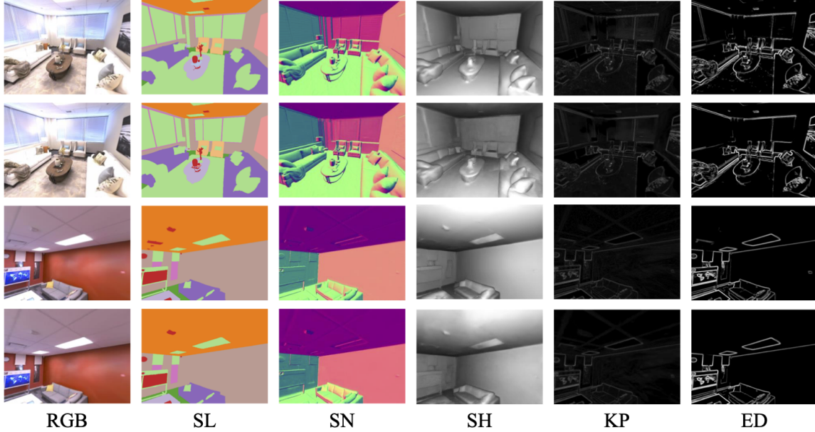
Figure 3: Qualitative results of two representative testing views on Replica. Top row: ground-truth; Bottom row: our synthesis results. The synthesized RGB images are from the SL task. SS-NeRF is able to render realistic and matched RGB images and other properties.
