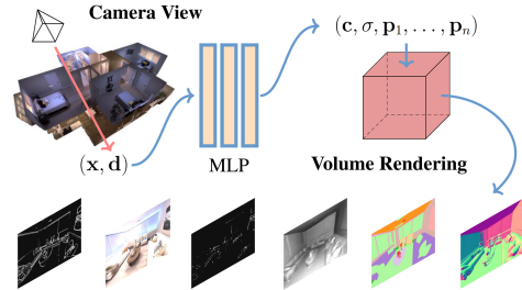
Figure 1: We represent the scene as an implicit function and develop a versatile neural scene representation, SS-NeRF, that is able to not only render images from novel viewpoints, but also render various scene properties (e.g., appearance, geometry, and semantics) paired with the synthesized images, under a unified framework.
