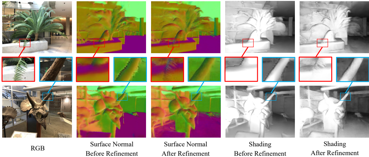
Figure 5: Surface normal and shading predictions with real-world images from the LLFF dataset. We use pre-trained annotators to obtain the initial labels which are noisy and flawed, and we retrain SS-NeRF with these labels. SS-NeRF can refine these flawed annotations and restore more details by joint modeling and understanding of the scenes.
