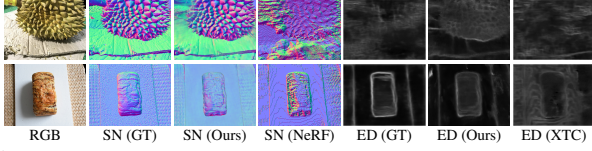
Figure 4: Representative results on blendedMVS. SN (NeRF) is the normal derived from NeRF’s depth; ED (XTC) is the edge predicted from a well-trained model taking NeRF’s normal as input. Our model outperforms both methods, indicating the capability and robustness of SS-NeRF.
