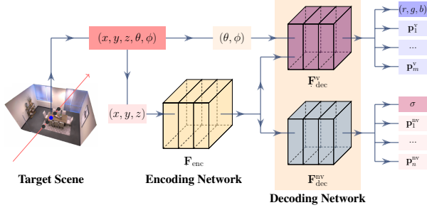
Figure 2: SS-NeRF architecture. The model takes the 3D coordinates and view directions as input and is able to synthesize different paired scene properties. SS-NeRF uses a shared scene encoding network F_{\text{enc}} to conduct the 3D positional embedding, followed by two separate decoding networks F_{\text{dec}}^v and F_{\text{dec}}^{nv} which produce scene property predictions. F_{\text{dec}}^v considers the view input, while F_{\text{dec}}^{nv} does not.
